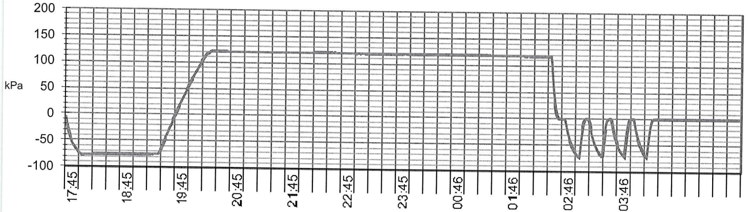
Pressure / Time graph - Pressure during exposure time : min 118 / MAX 120 kPa
