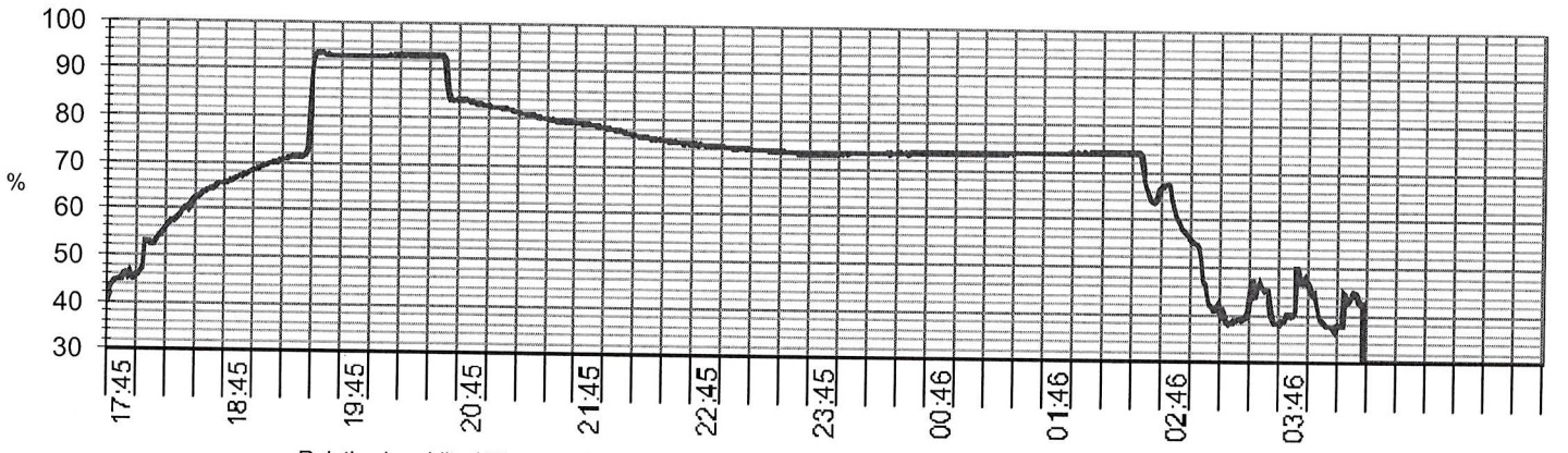
Relative humidity / Time graph - RH at the end of conditioning : 72 %, RH during exposure time : min 73 %
