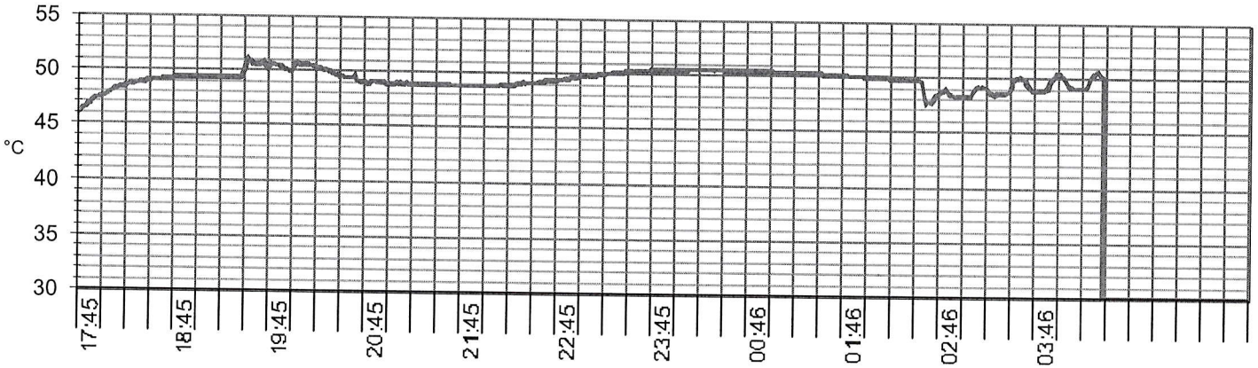
Temperature / Time graph - Temperature during exposure time : min 48,8 / MAX 50,5 °C
