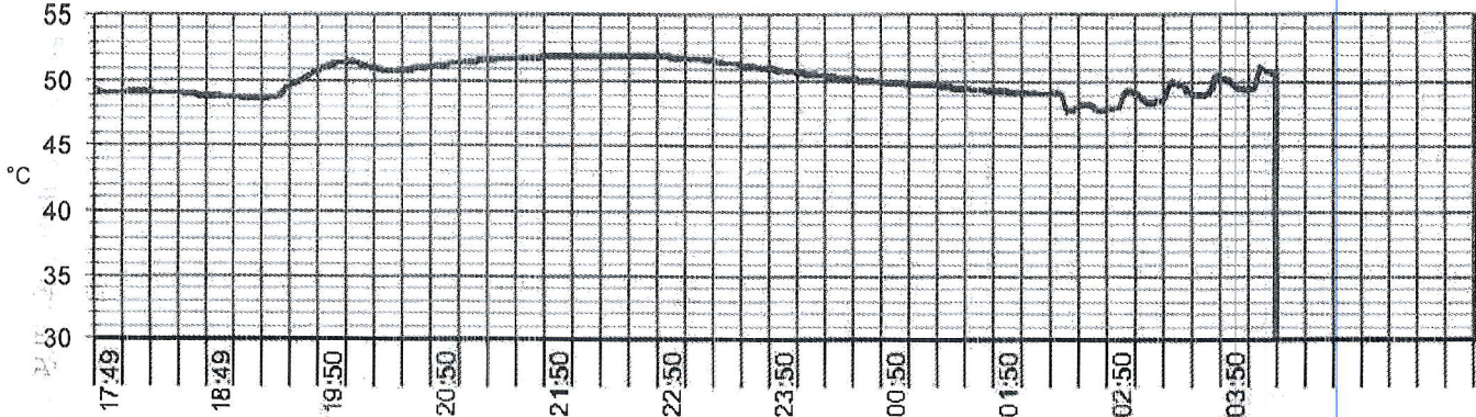
Temperature / Time graph - Temperature during exposure time : min 49,1 / MAX 52,0 °C
