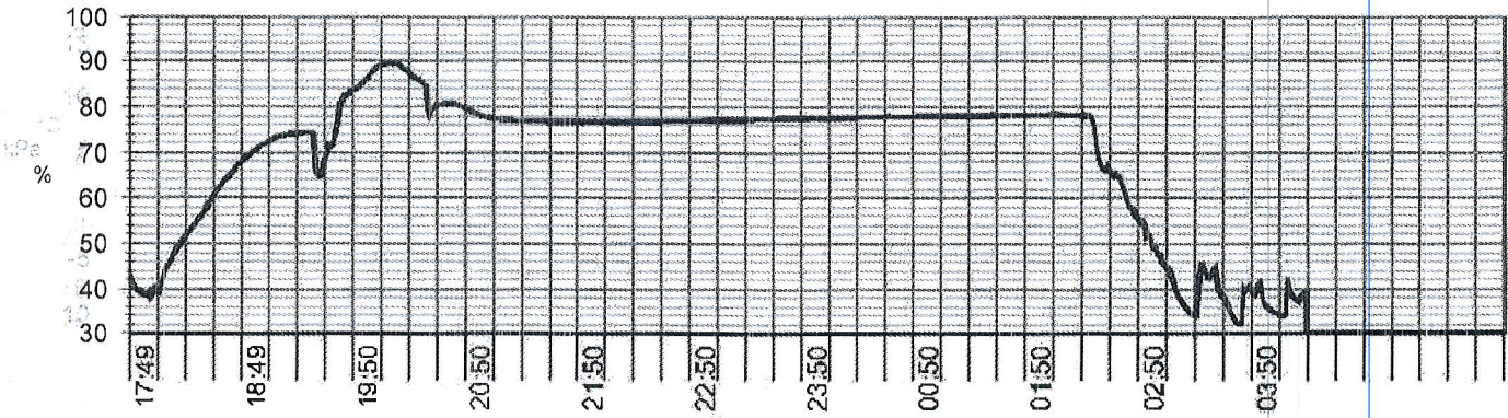
Relative humidity / Time graph - RH at the end of conditioning : 74 %, RH during exposure time : min 77 %
