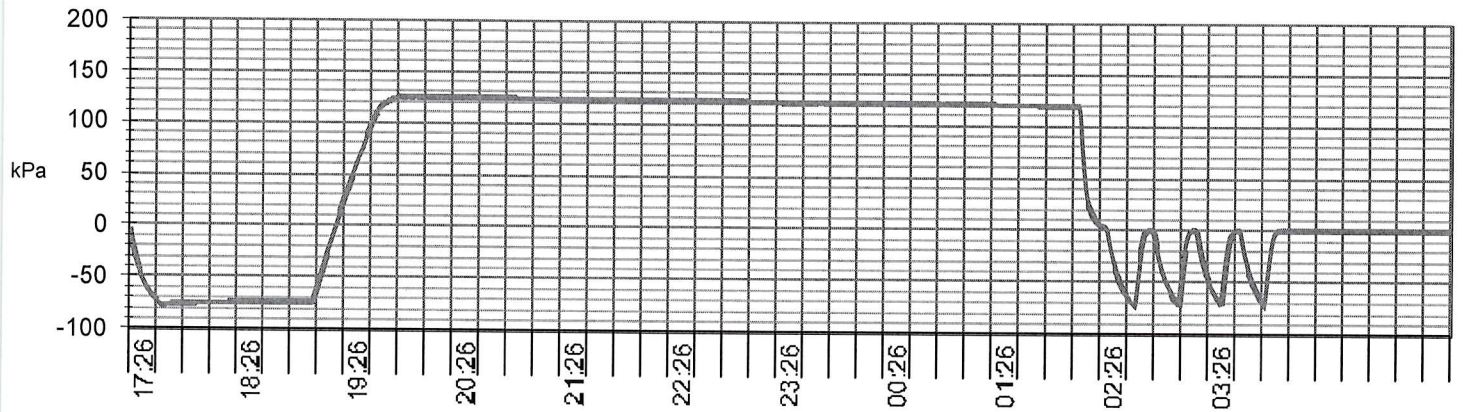
Pressure / Time graph - Pressure during exposure time : min 119 / MAX 124 kPa
