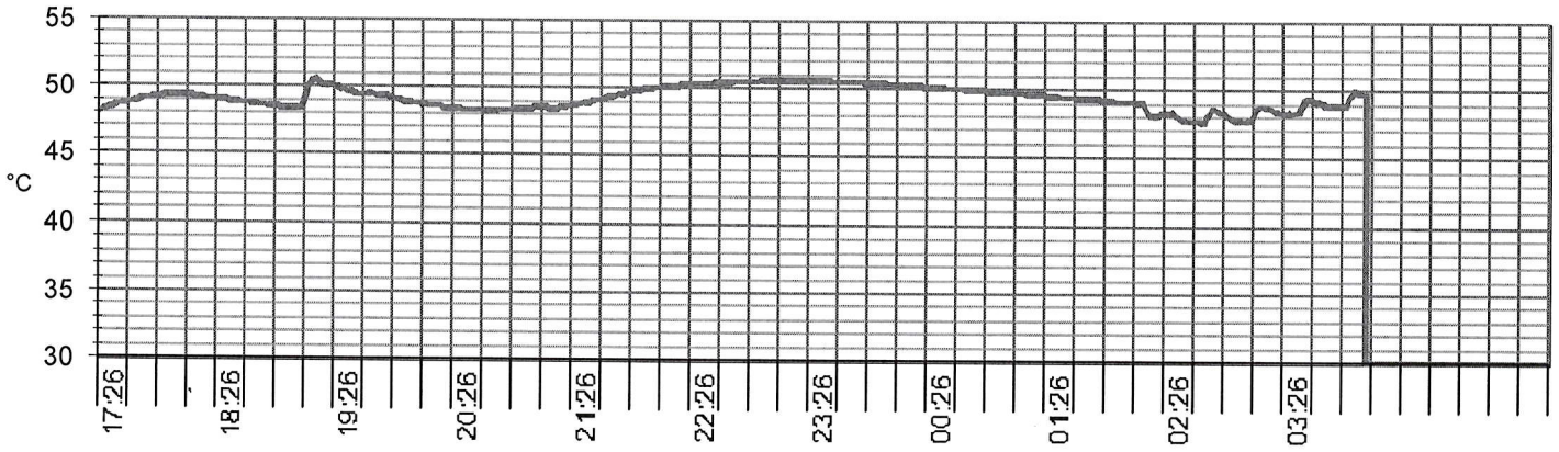
Temperature / Time graph - Temperature during exposure time : min 48,2 / MAX 50,6 °C
