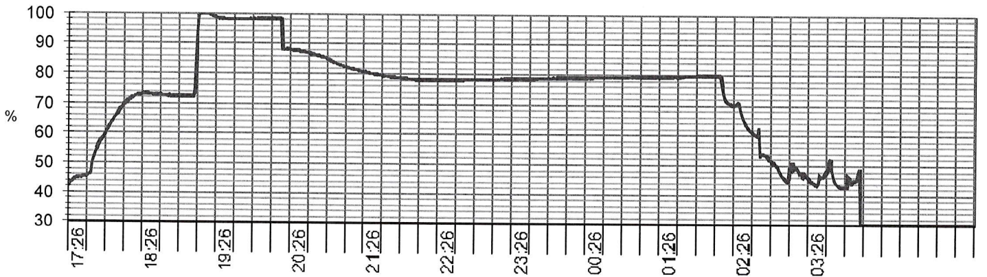
Relative humidity / Time graph - RH at the end of conditioning : 72 %, RH during exposure time : min 78 %
