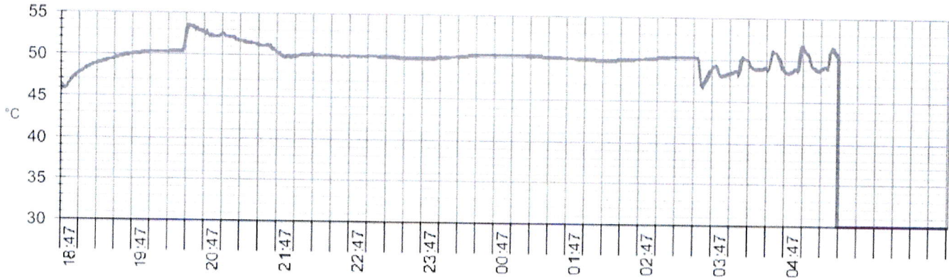
Temperature / Time graph - Temperature during exposure time : min 49.7 / MAX 51.2 °C
