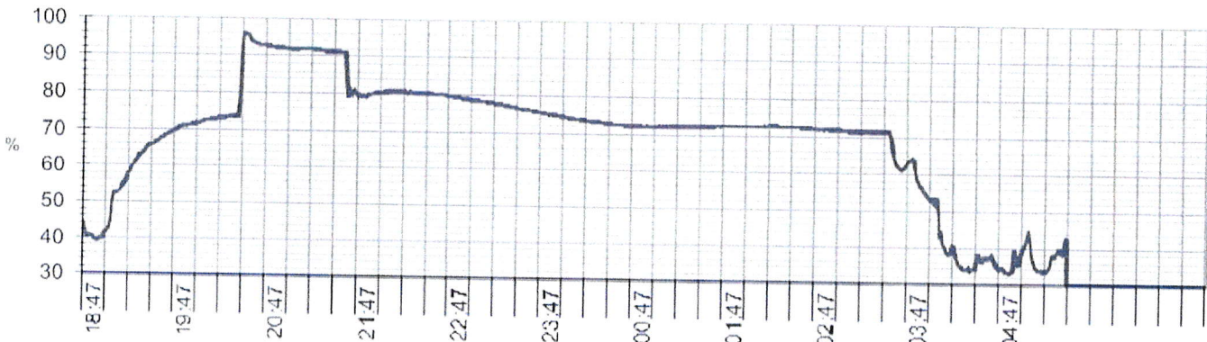
Relative humidity / Time graph - RH at the end of conditioning : 74 %, RH during exposure time : min 71 %
